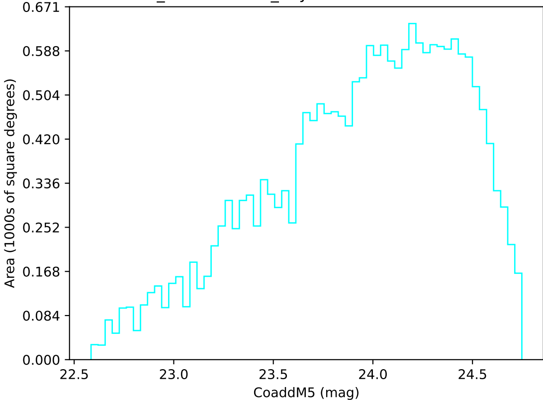
weather_cloudso1v3.4_10yrs Yr 3-4 u band: CoaddM5
