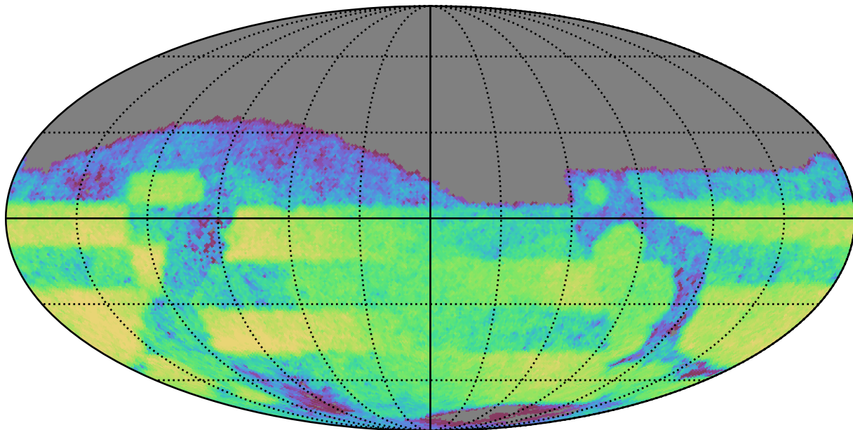
weather_cloudso1v3.4_10yrs Yr 3-4 r band: CoaddM5
