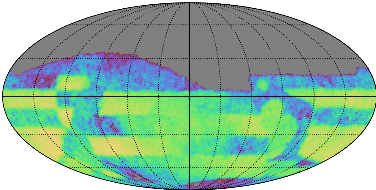
weather_cloudso1v3.4_10yrs Yr 3-4 i band: CoaddM5
