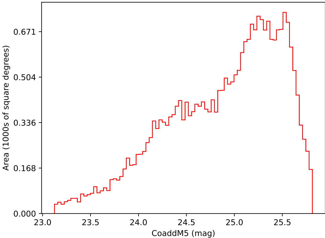
weather_cloudso1v3.4_10yrs Yr 3-4 i band: CoaddM5
