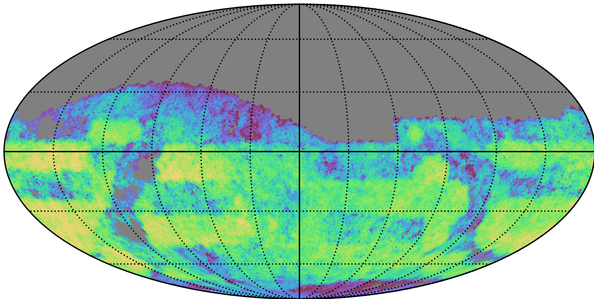
weather_cloudso1v3.4_10yrs Yr 3-4 g band: CoaddM5
