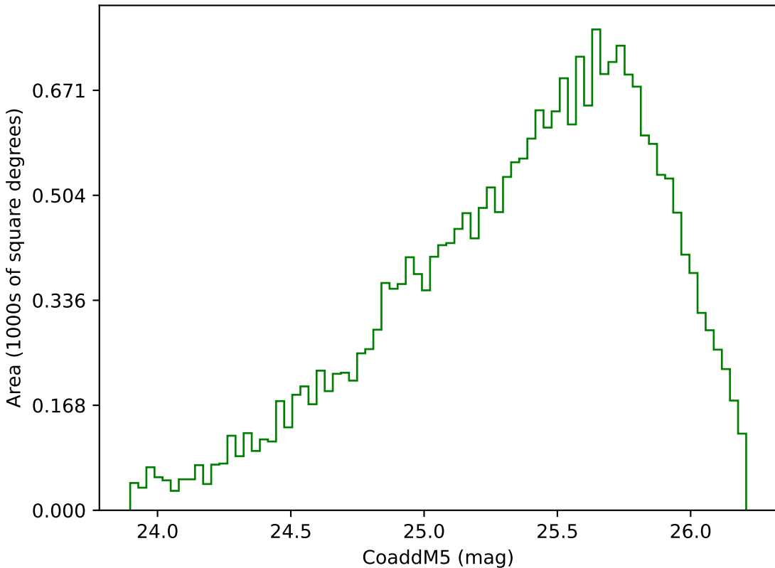
weather_cloudso1v3.4_10yrs Yr 3-4 g band: CoaddM5
