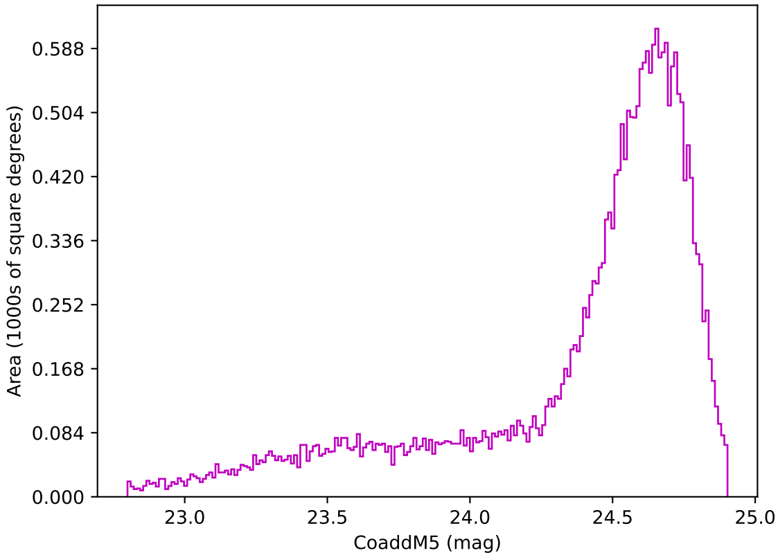
weather_cloudso1v3.4_10yrs Yr 1 z band: CoaddM5
