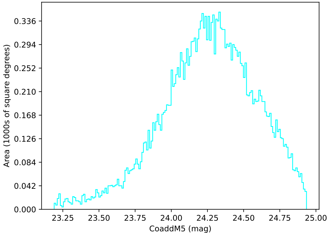
weather_cloudso1v3.4_10yrs Yr 1 u band: CoaddM5
