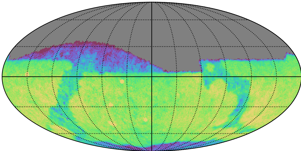
weather_cloudso1v3.4_10yrs Yr 1 r band: CoaddM5
