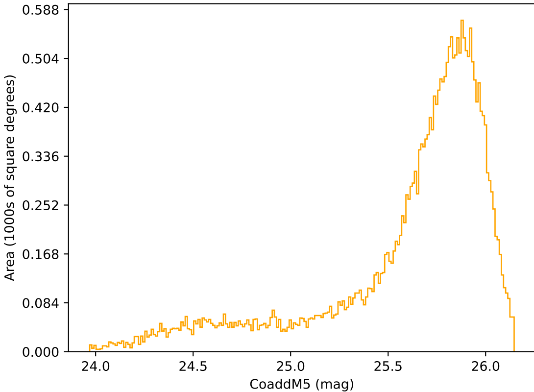
weather_cloudso1v3.4_10yrs Yr 1 r band: CoaddM5
