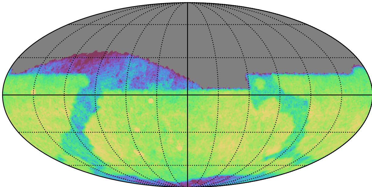
weather_cloudso1v3.4_10yrs Yr 1 i band: CoaddM5
