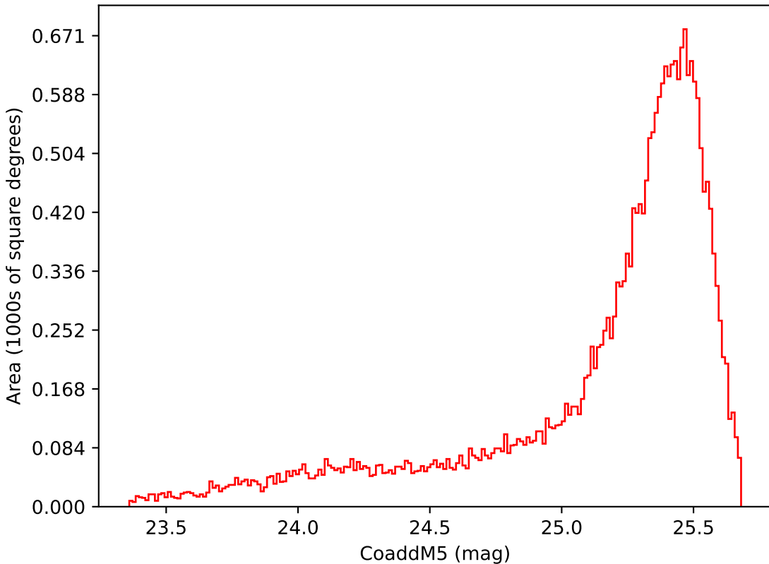
weather_cloudso1v3.4_10yrs Yr 1 i band: CoaddM5
