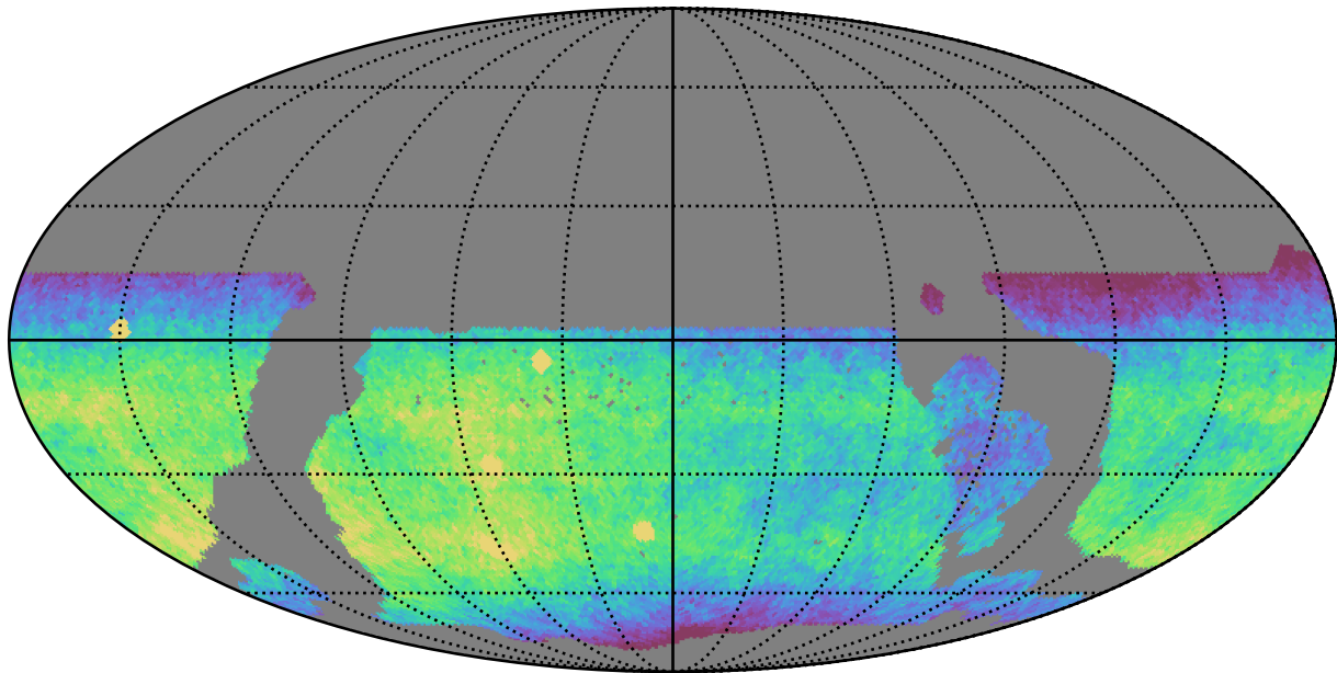
weather_cloudso1v3.4_10yrs WFD z band: CoaddM5
