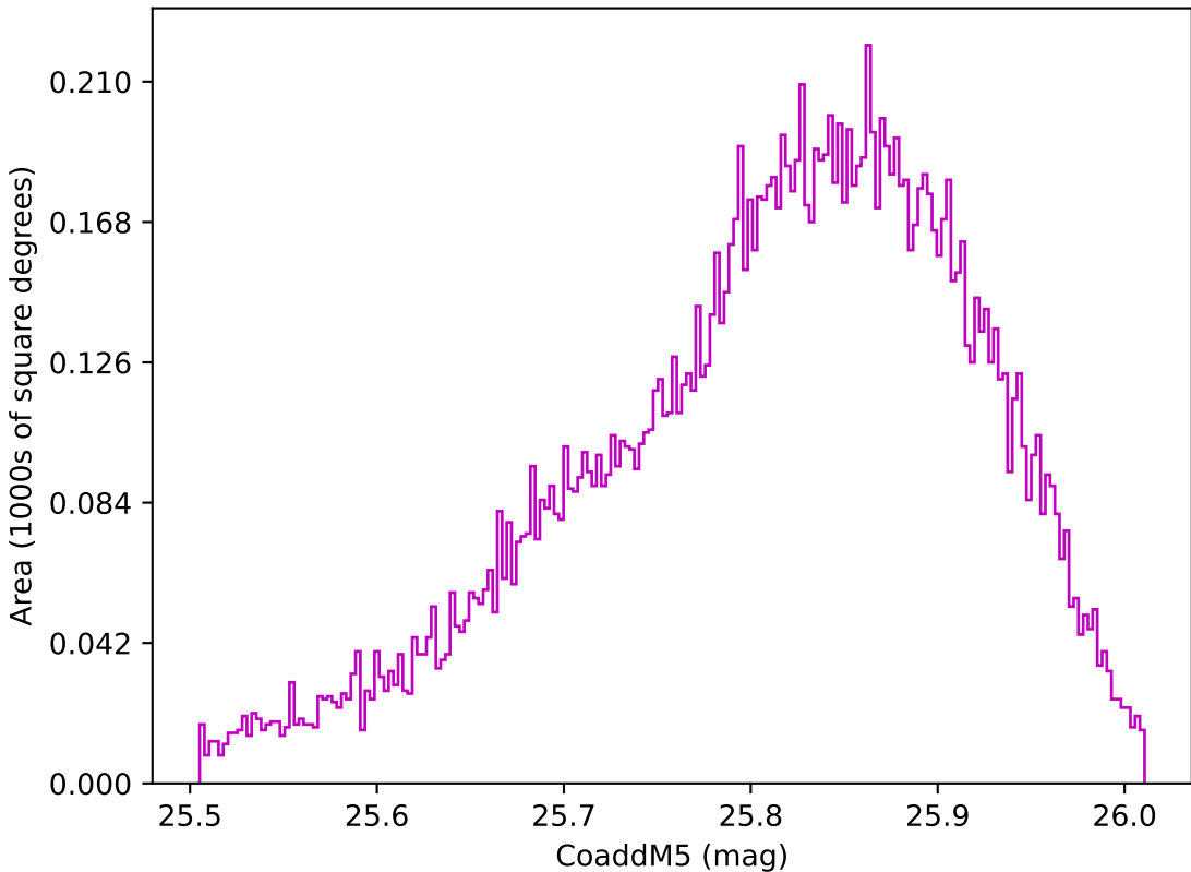
weather_cloudso1v3.4_10yrs WFD z band: CoaddM5
