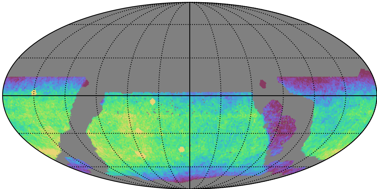
weather_cloudso1v3.4_10yrs WFD y band: CoaddM5
