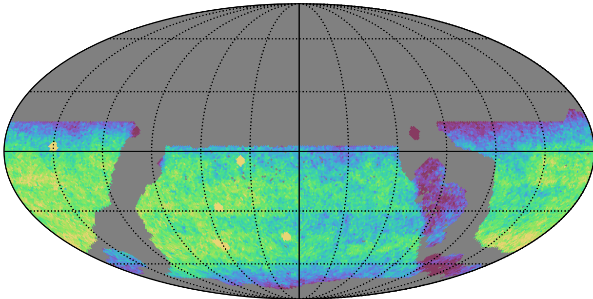
weather_cloudso1v3.4_10yrs WFD u band: CoaddM5
