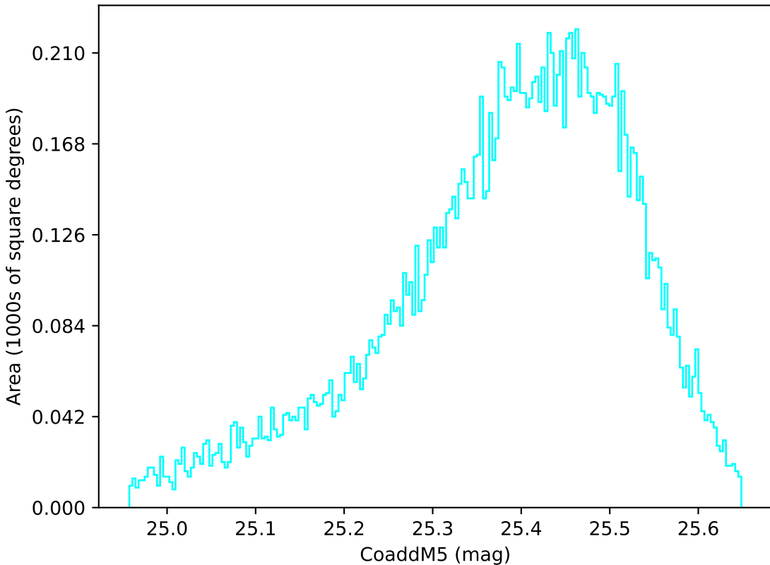
weather_cloudso1v3.4_10yrs WFD u band: CoaddM5
