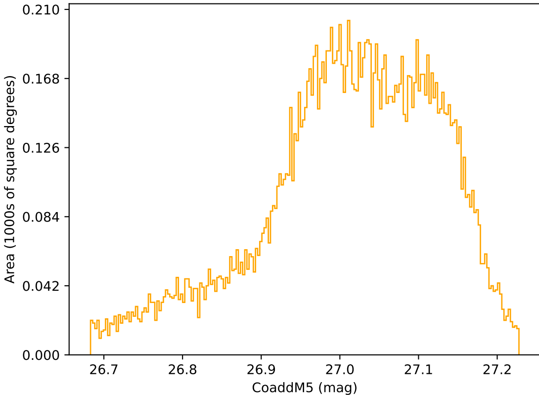
weather_cloudso1v3.4_10yrs WFD r band: CoaddM5
