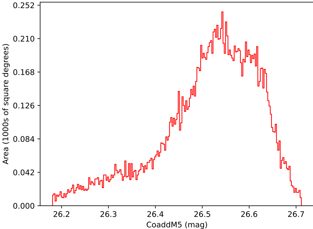
weather_cloudso1v3.4_10yrs WFD i band: CoaddM5
