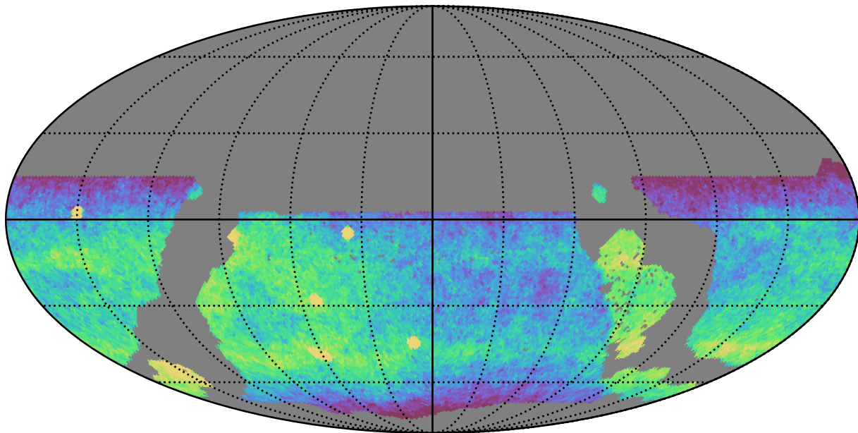
weather_cloudso1v3.4_10yrs WFD g band: CoaddM5
