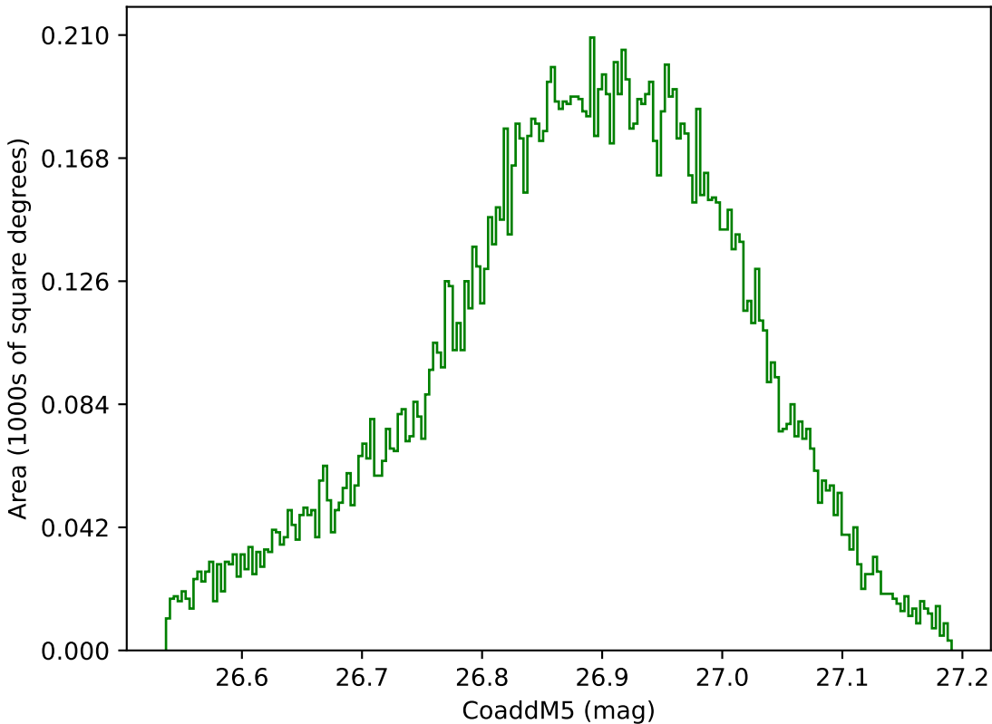
weather_cloudso1v3.4_10yrs WFD g band: CoaddM5
