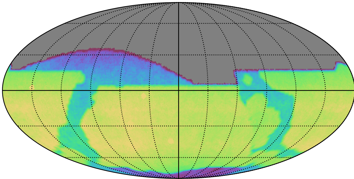
weather_cloudso1v3.4_10yrs All sky z band: CoaddM5
