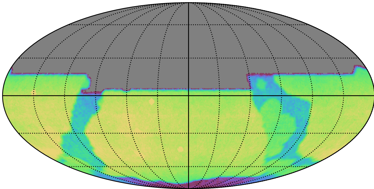
weather_cloudso1v3.4_10yrs All sky y band: CoaddM5
