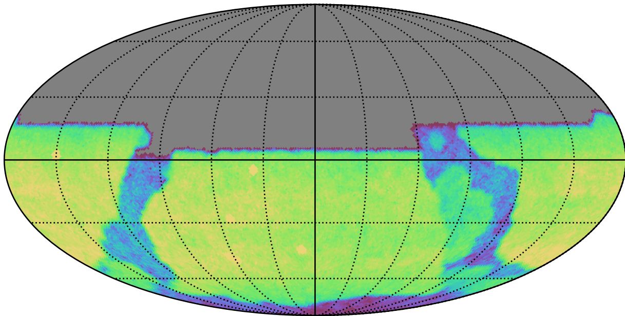
weather_cloudso1v3.4_10yrs All sky u band: CoaddM5
