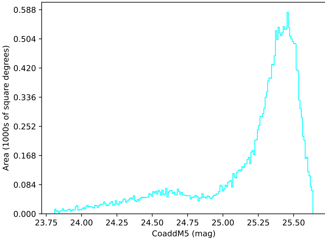
weather_cloudso1v3.4_10yrs All sky u band: CoaddM5
