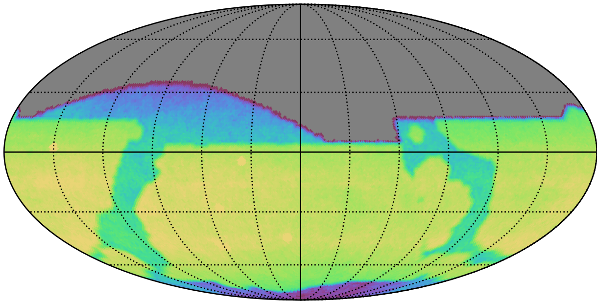
weather_cloudso1v3.4_10yrs All sky i band: CoaddM5
