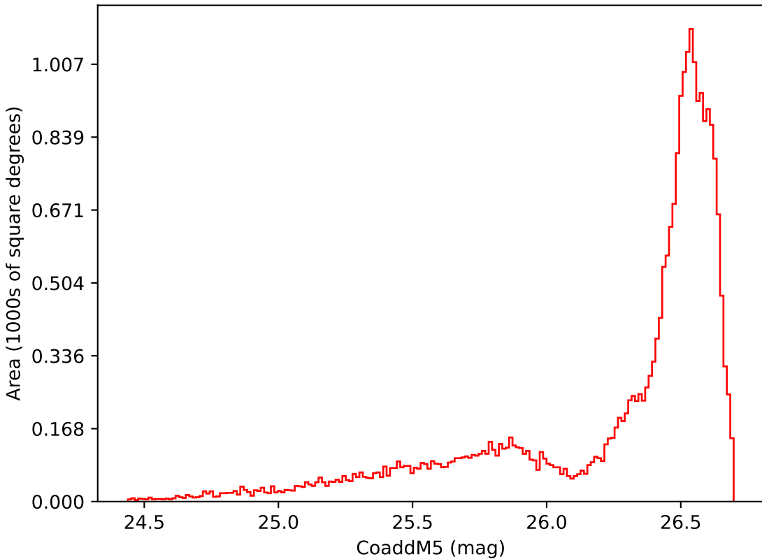
weather_cloudso1v3.4_10yrs All sky i band: CoaddM5
