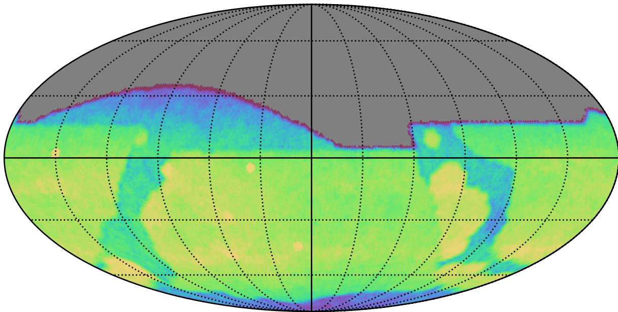
weather_cloudso1v3.4_10yrs All sky g band: CoaddM5
