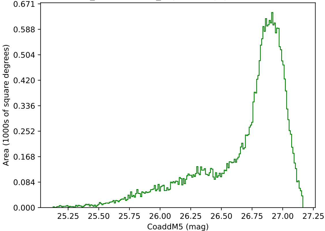
weather_cloudso1v3.4_10yrs All sky g band: CoaddM5
