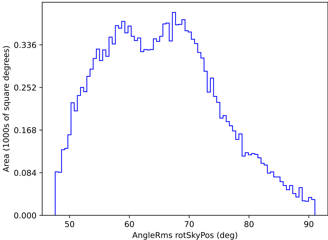
weather_cloudso1v3.4_10yrs WFD z band: AngleRms rotSkyPos
