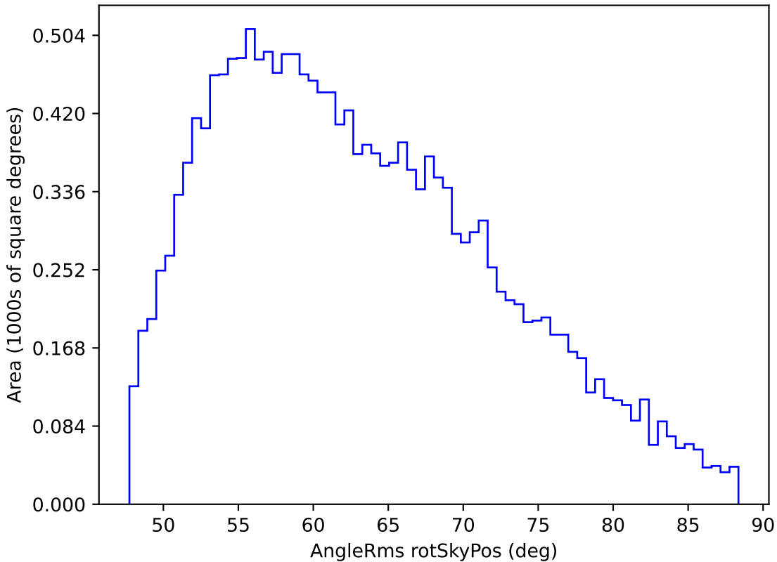
weather_cloudso1v3.4_10yrs WFD y band: AngleRms rotSkyPos
