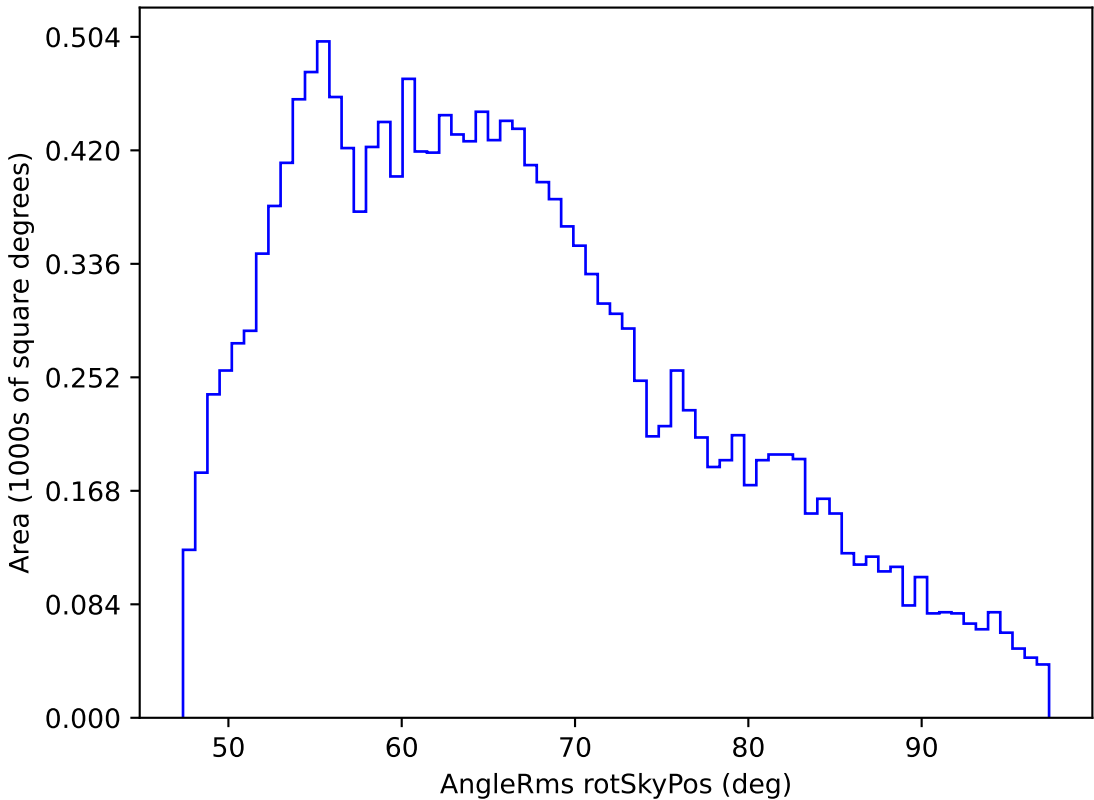
weather_cloudso1v3.4_10yrs WFD r band: AngleRms rotSkyPos
