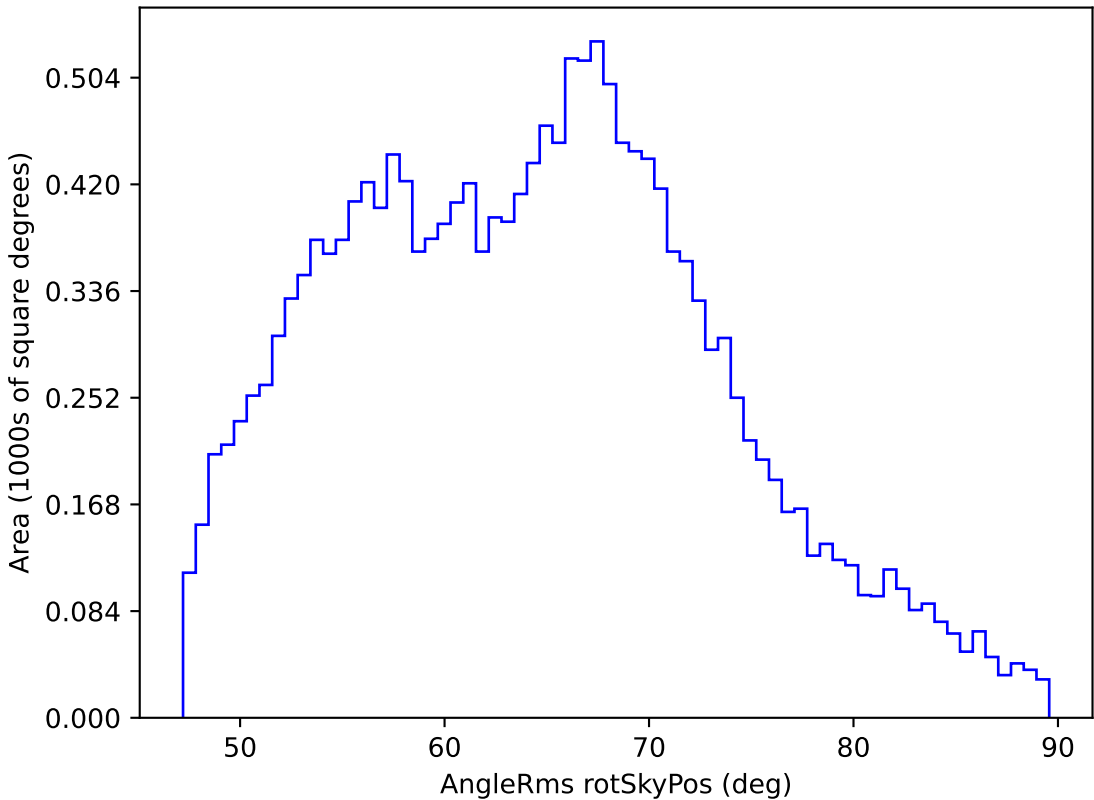
weather_cloudso1v3.4_10yrs WFD i band: AngleRms rotSkyPos
