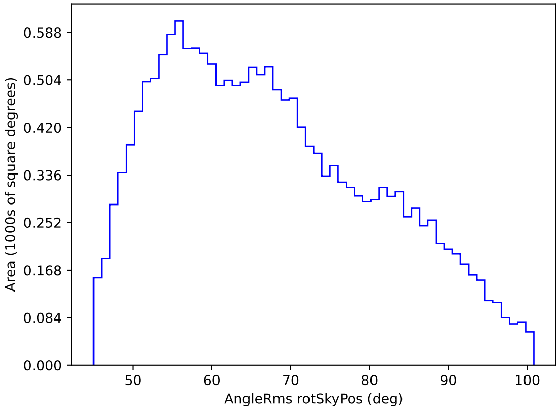
weather_cloudso1v3.4_10yrs WFD g band: AngleRms rotSkyPos
