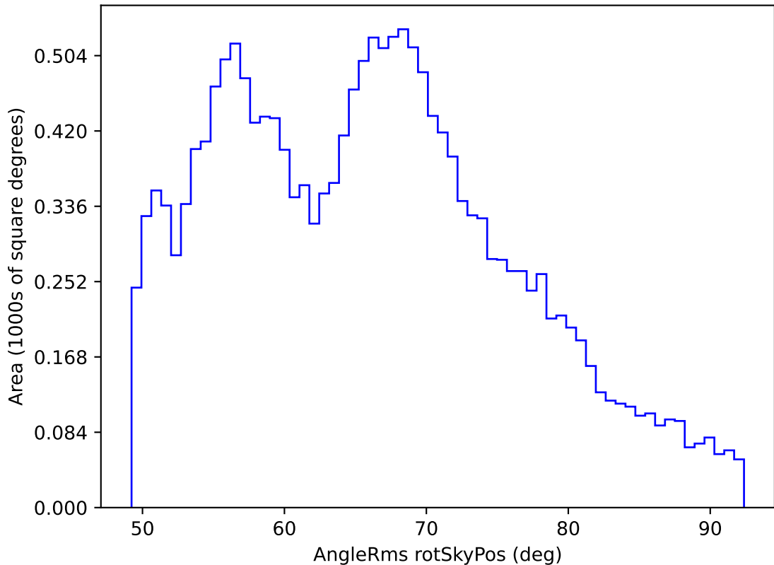
weather_cloudso1v3.4_10yrs WFD all bands: AngleRms rotSkyPos
