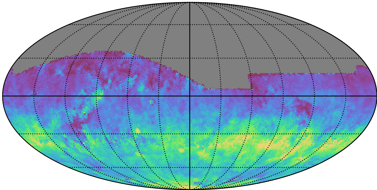
weather_cloudso1v3.4_10yrs All sky z band: AngleRms rotSkyPos
