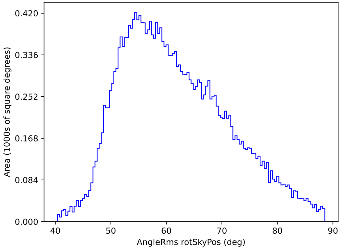
weather_cloudso1v3.4_10yrs All sky y band: AngleRms rotSkyPos
