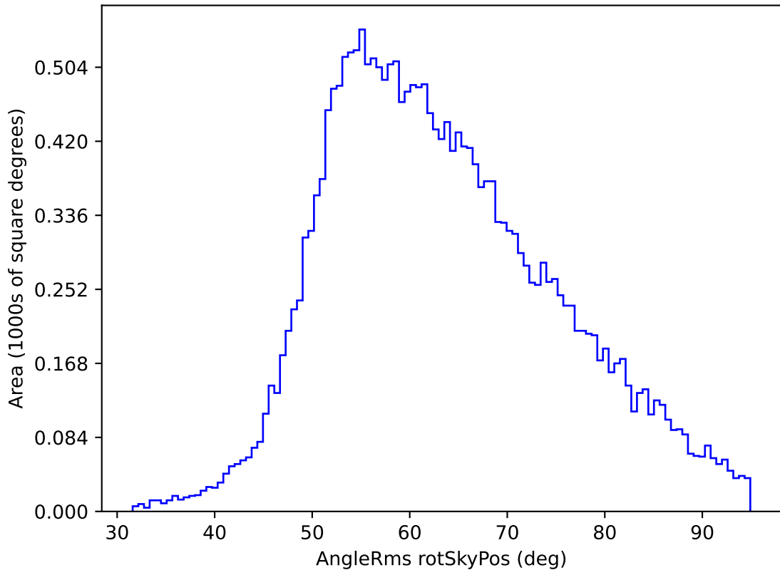
weather_cloudso1v3.4_10yrs All sky u band: AngleRms rotSkyPos
