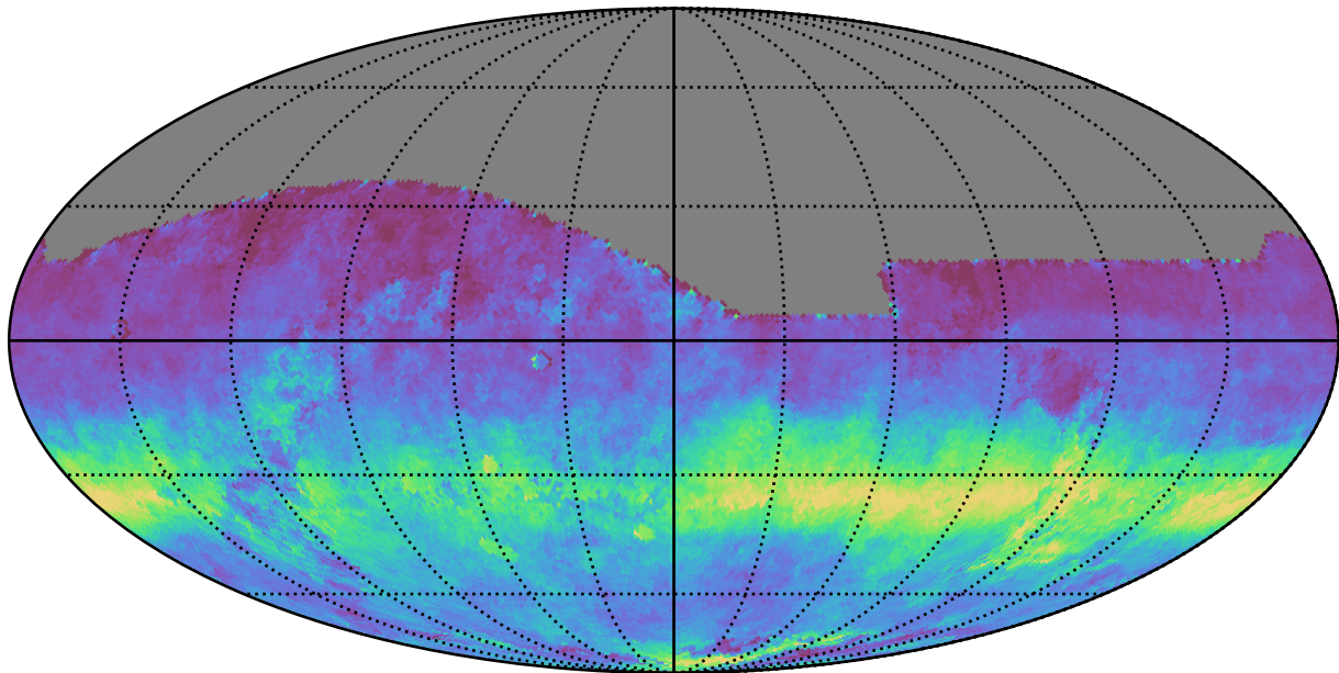
weather_cloudso1v3.4_10yrs All sky r band: AngleRms rotSkyPos
