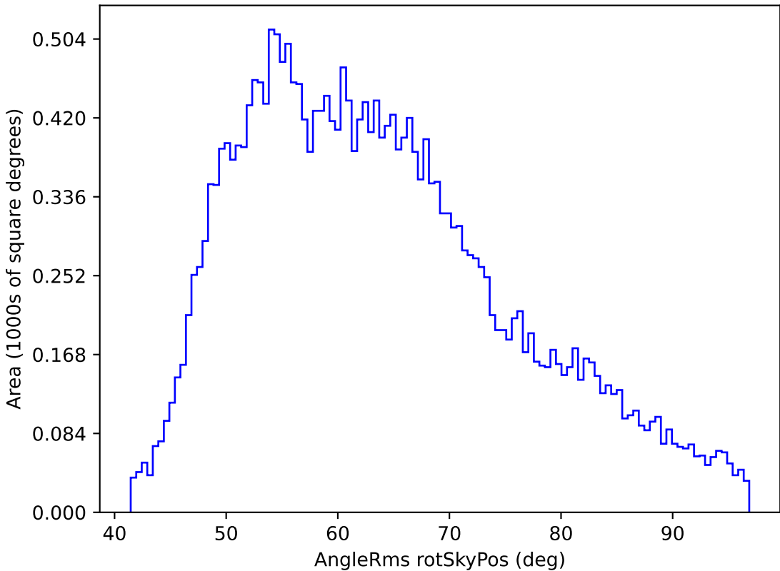
weather_cloudso1v3.4_10yrs All sky r band: AngleRms rotSkyPos
