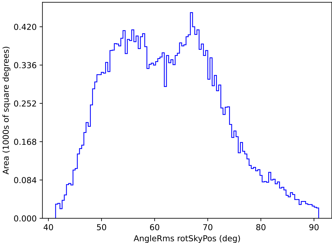
weather_cloudso1v3.4_10yrs All sky i band: AngleRms rotSkyPos
