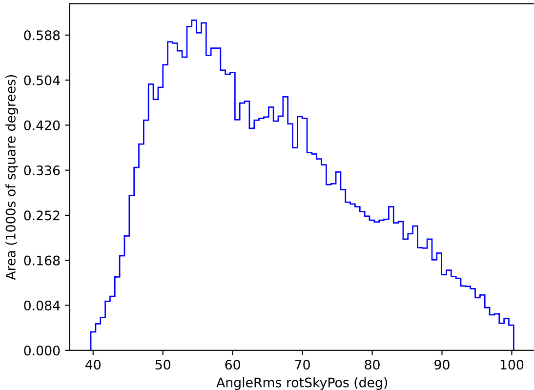
weather_cloudso1v3.4_10yrs All sky g band: AngleRms rotSkyPos
