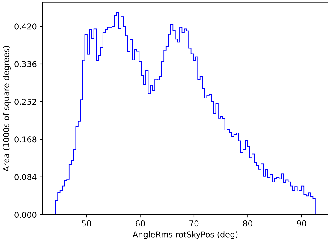
weather_cloudso1v3.4_10yrs All sky all bands: AngleRms rotSkyPos
