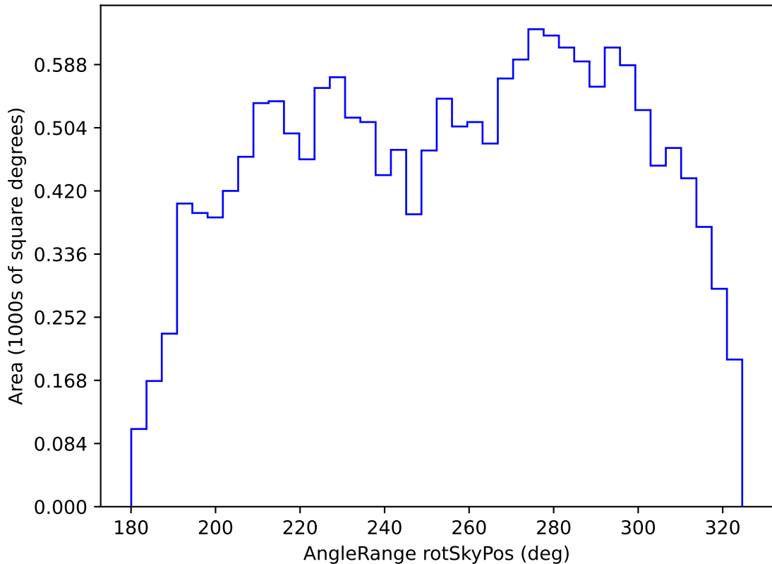
weather_cloudso1v3.4_10yrs WFD u band: AngleRange rotSkyPos
