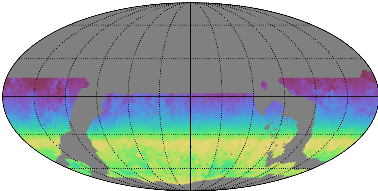
weather_cloudso1v3.4_10yrs WFD all bands: AngleRange rotSkyPos
