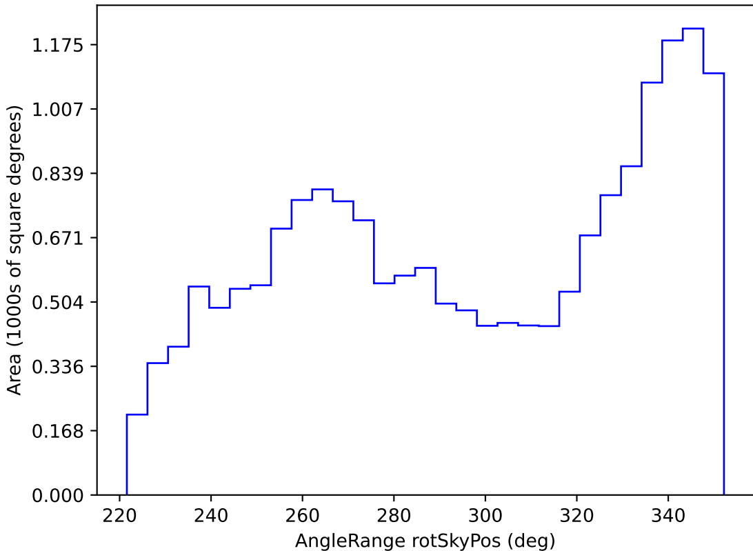
weather_cloudso1v3.4_10yrs WFD all bands: AngleRange rotSkyPos
