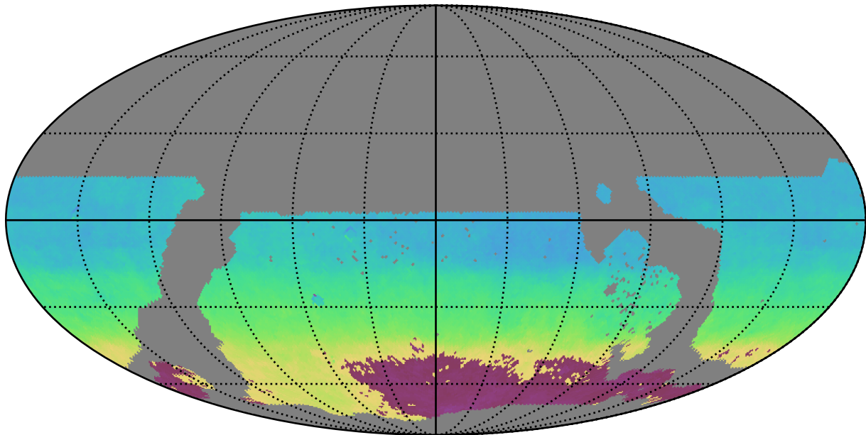
weather_cloudso1v3.4_10yrs WFD z band: AngleMean rotSkyPos
