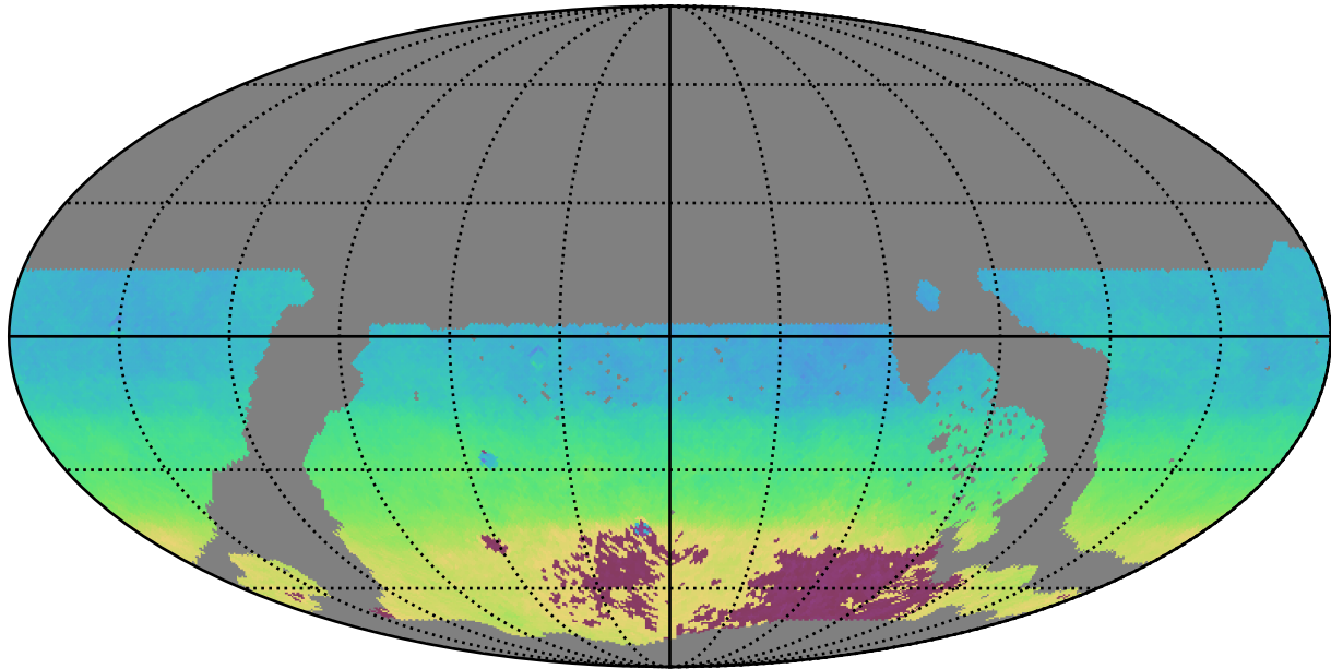
weather_cloudso1v3.4_10yrs WFD y band: AngleMean rotSkyPos
