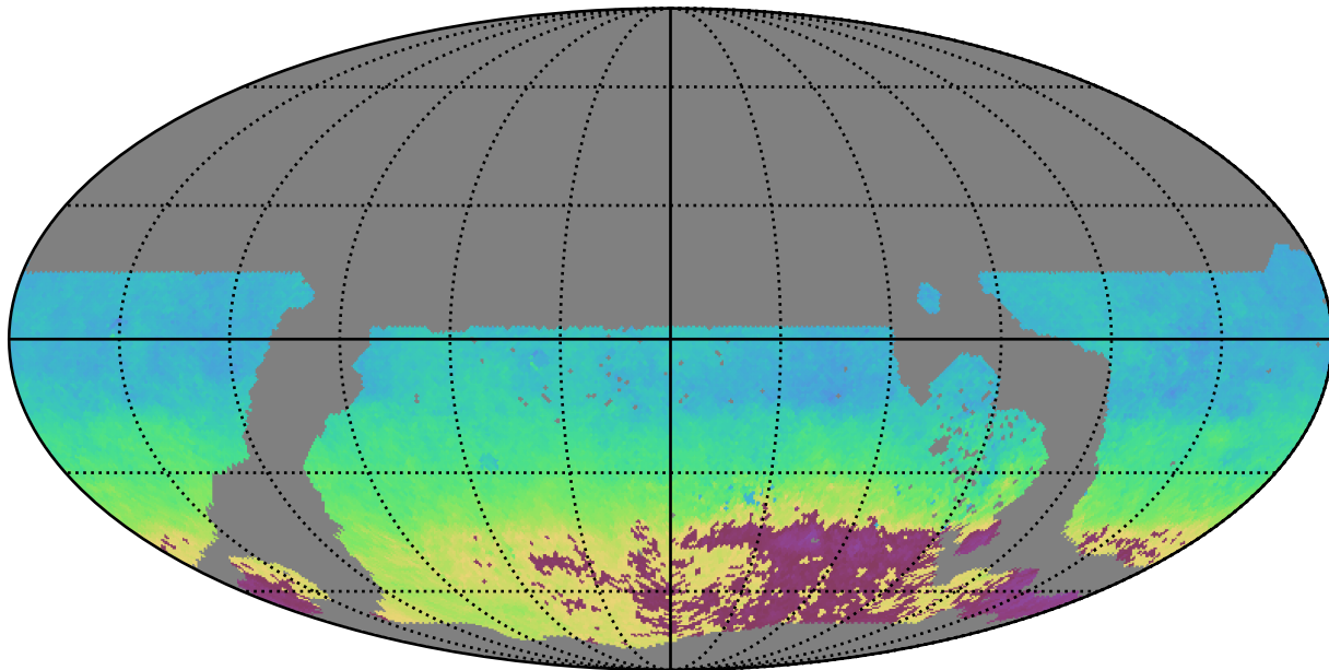
weather_cloudso1v3.4_10yrs WFD u band: AngleMean rotSkyPos
