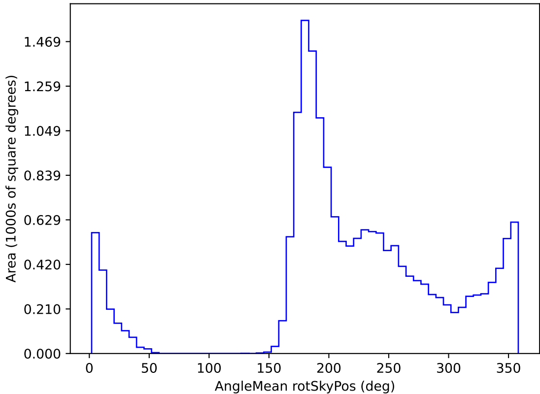
weather_cloudso1v3.4_10yrs WFD u band: AngleMean rotSkyPos
